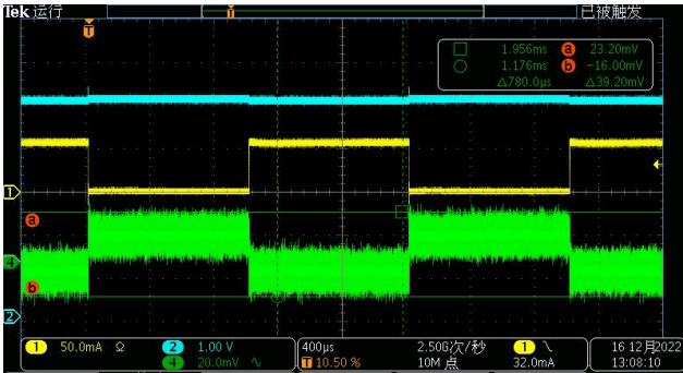
VBAT=VKEY=36V, I_{12V}=60\text{mA} 图 9-25 12V 负载调整
