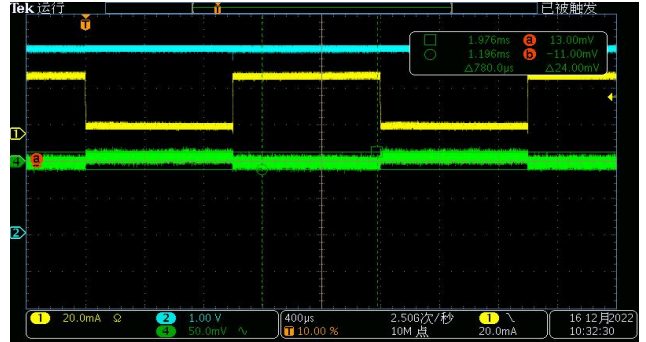
VBAT=VKEY=36V, I_{5V}=30\text{mA} 图 9-26 5V 负载调整
