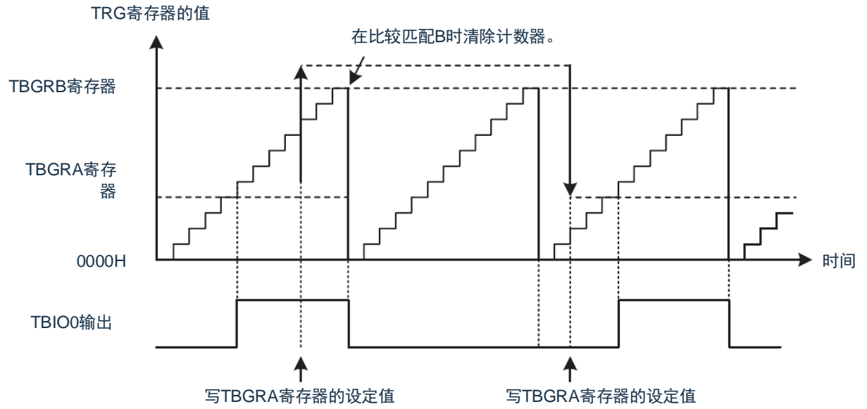
(a) 占空比0%
