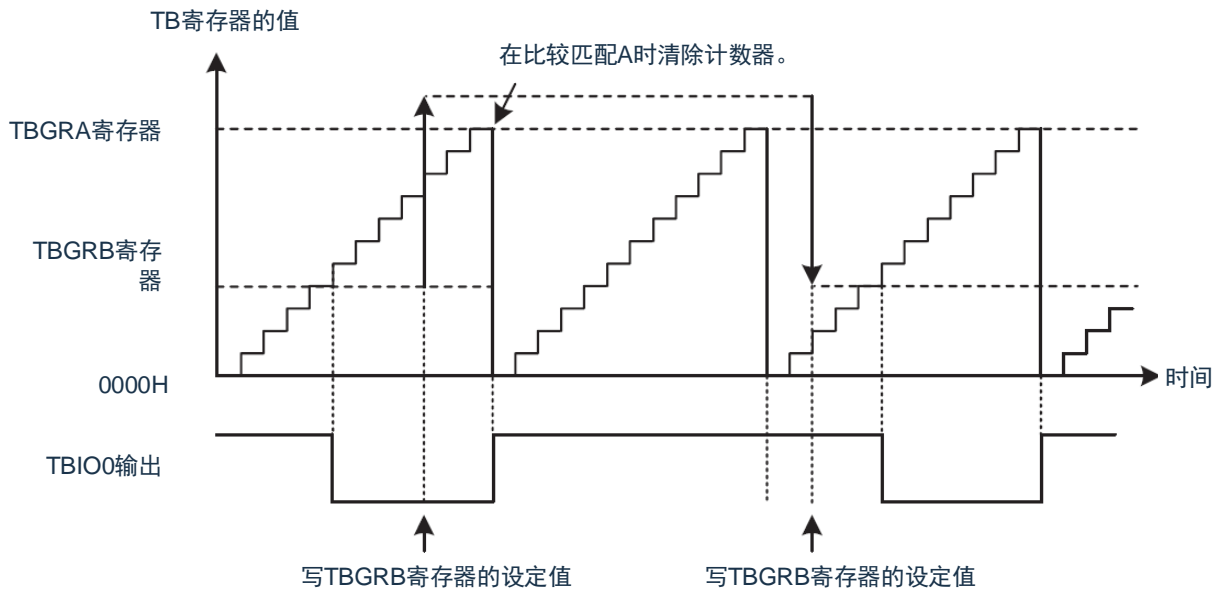
(b) 占空比100%
